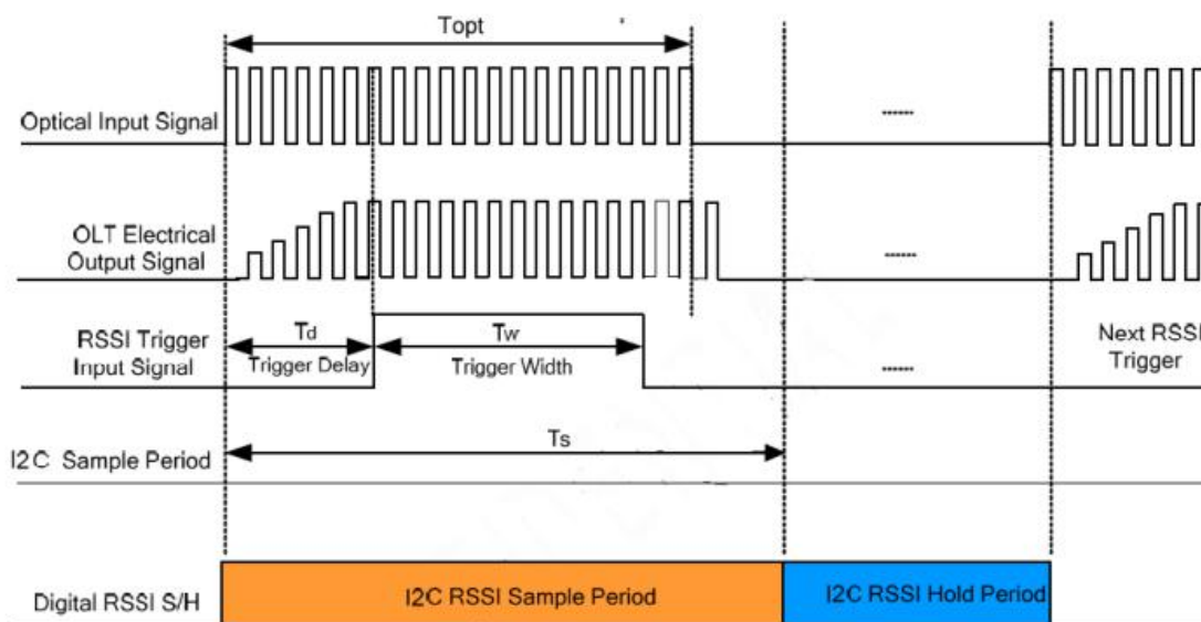
Figure 4 Timing Parameter Definitions in RSSI Trigger
