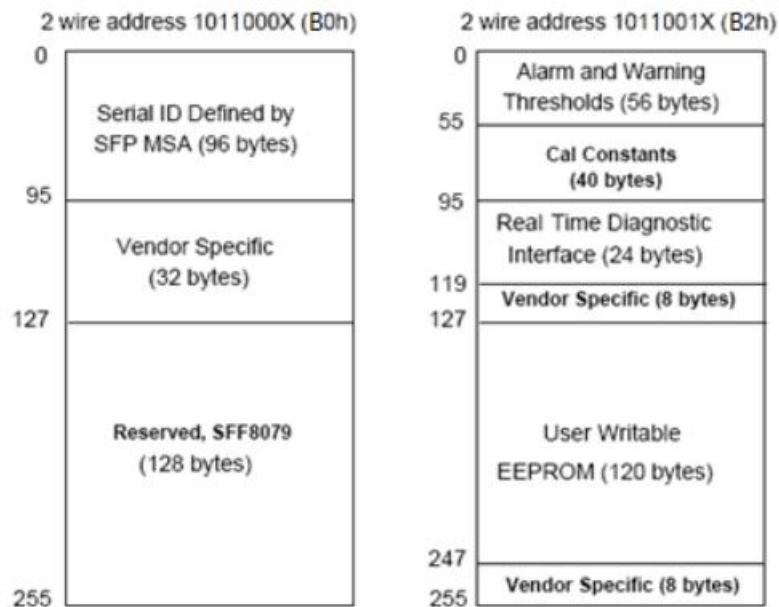
Figure 6: EEPROM Memory Map Specific Data Field Description
