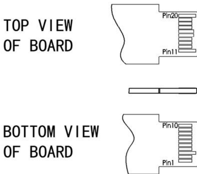
Figure 5: Pin Out Drawing
