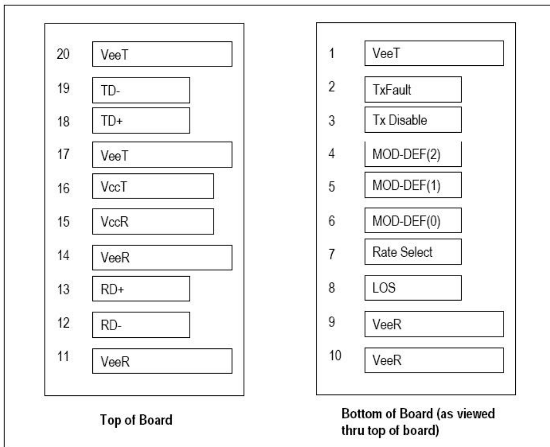
Figure 3 Pin Out Drawing (Top view)
