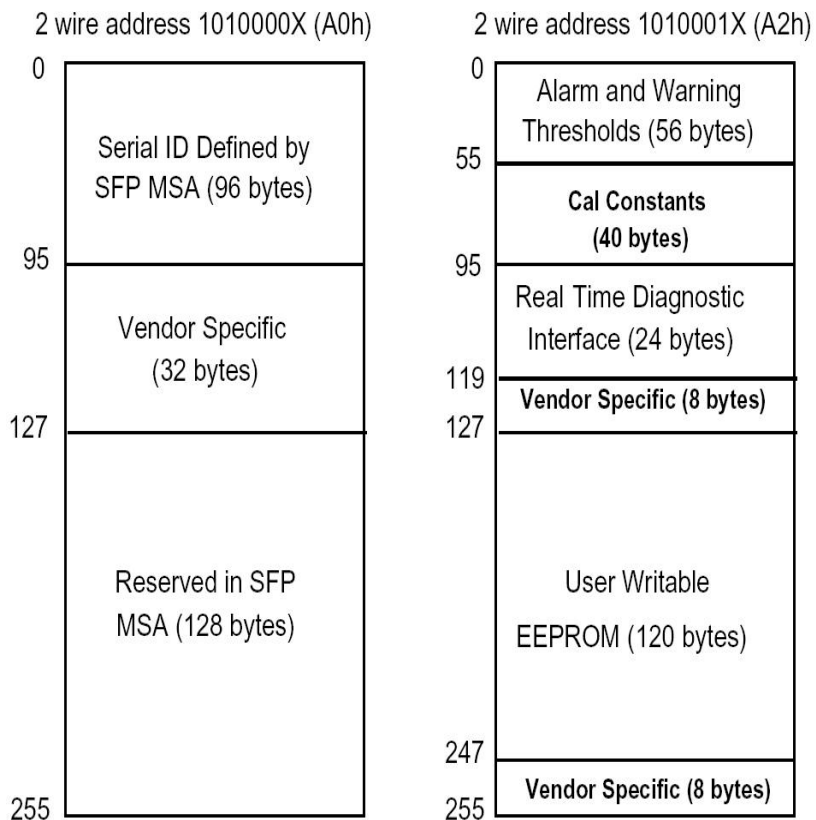
Figure 2 EEPROM Information
