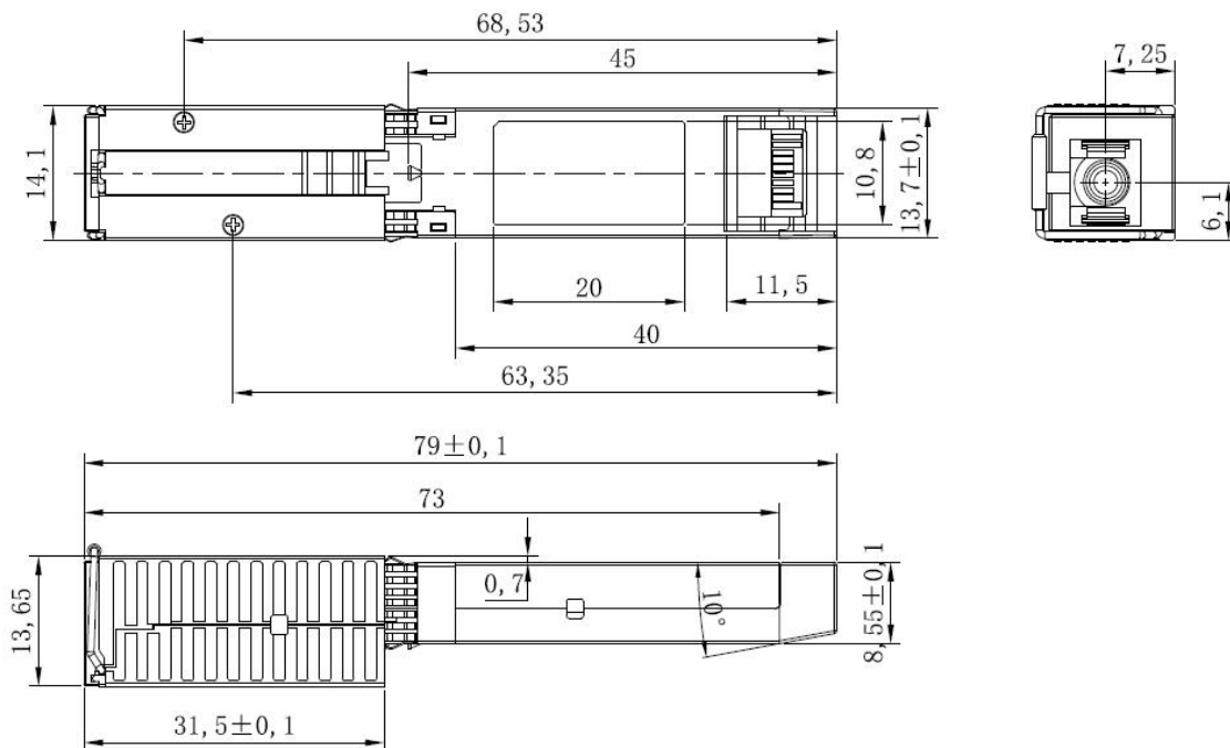
Figure 5 Package Outline (unit: mm)
