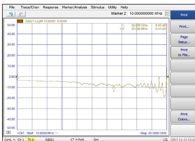
SDD21-3.5dB (Transmit Insertion Loss )
