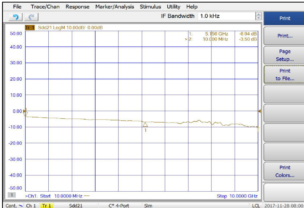
SDD21-3.5dB (Transmit Insertion Loss )
