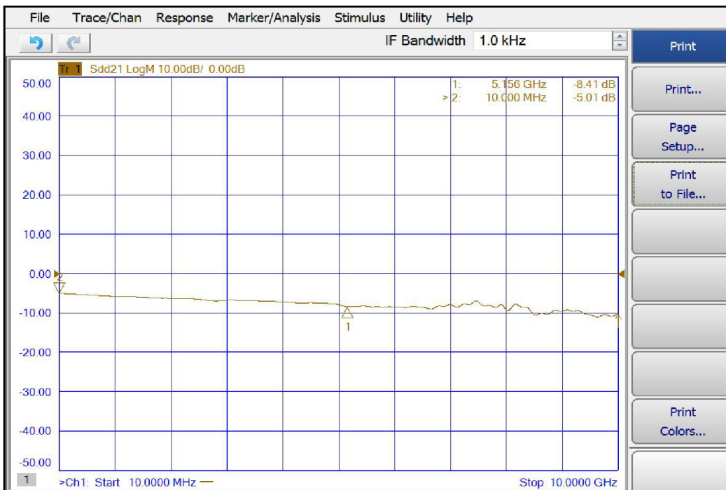
SDD21-5dB (Transmit Insertion Loss )
