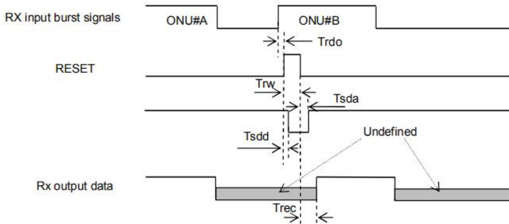
Figure 2: Timing Parameter Definitions in Burst Mode Sequence
