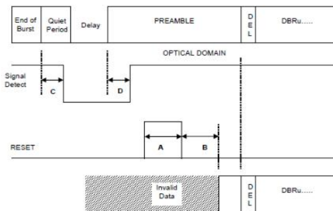
Figure 2: Reset Signal Timing Diagram in Normal Mode
