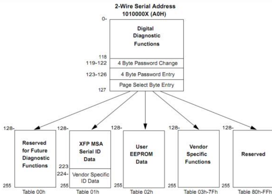
Figure 7: EEPROM Memory Map Specific Data Field Descriptions
