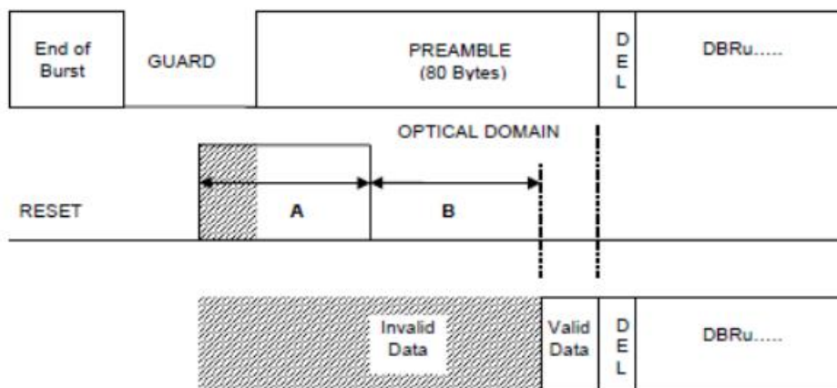
Figure 3: Reset Signal Timing Diagram in Ranging Mode
