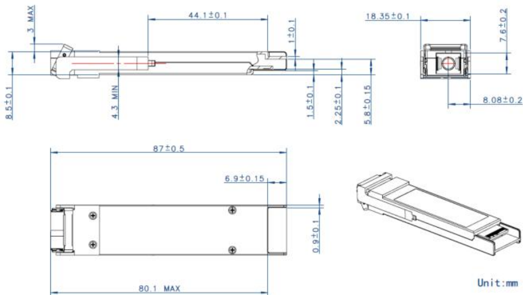
Figure 8: Package Outline
