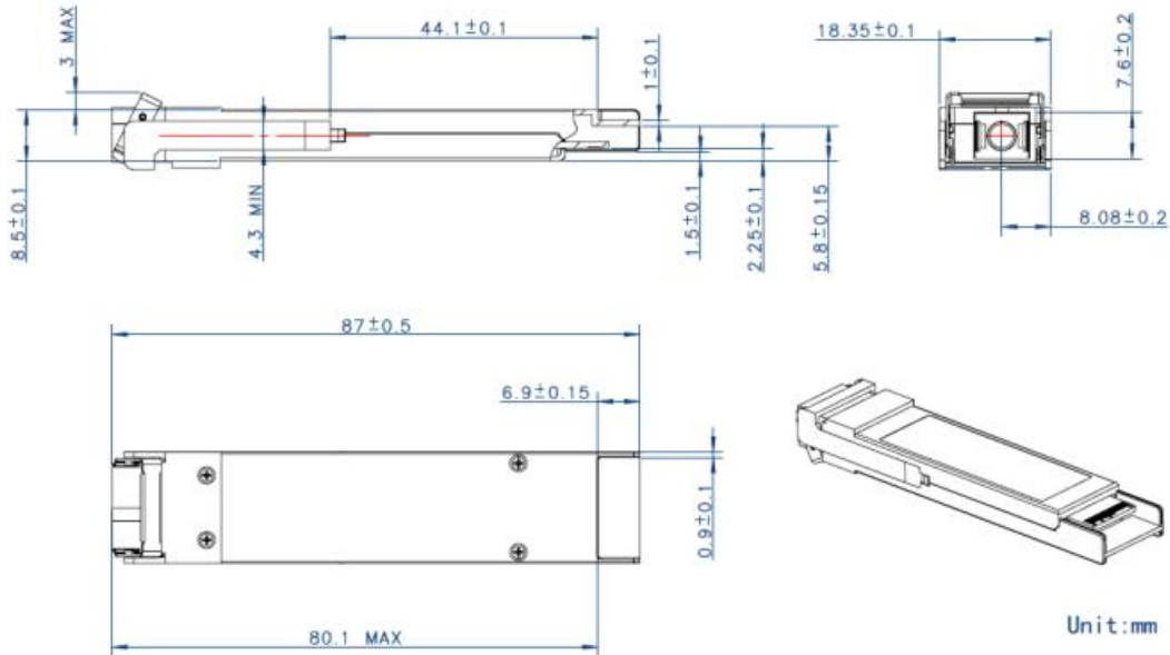
Figure 8: Package Outline
